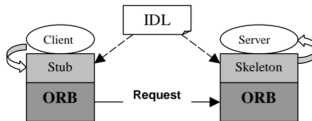
Figure 5. Stub and skeleton files
