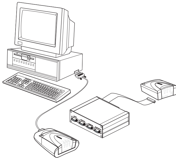
Figure 3. Nokia M2M ADK set-up
