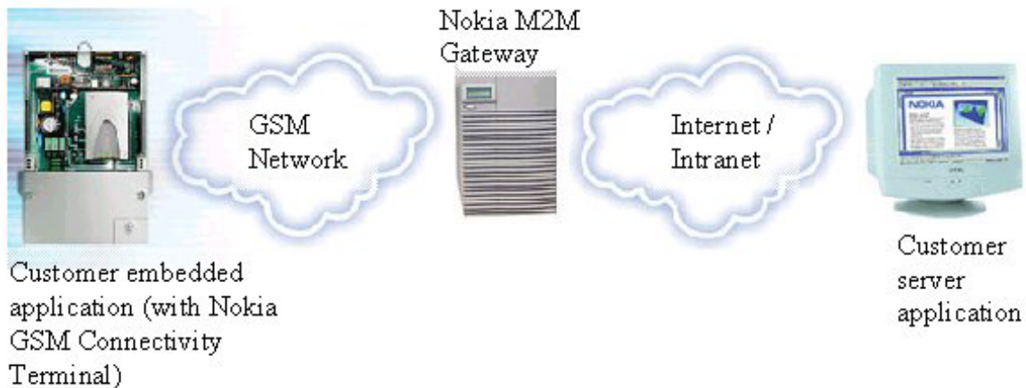
Figure 1. Nokia M2M Platform
