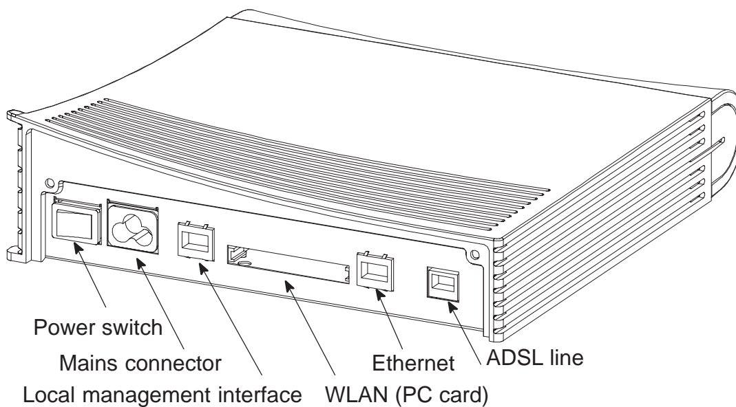
Figure 2 MW1122 back panel
