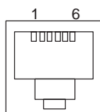
Figure 22 DSL connector
