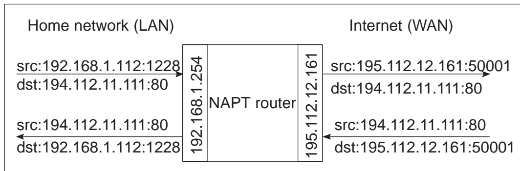
Figure 19 Principle of Network Address Port Translation
