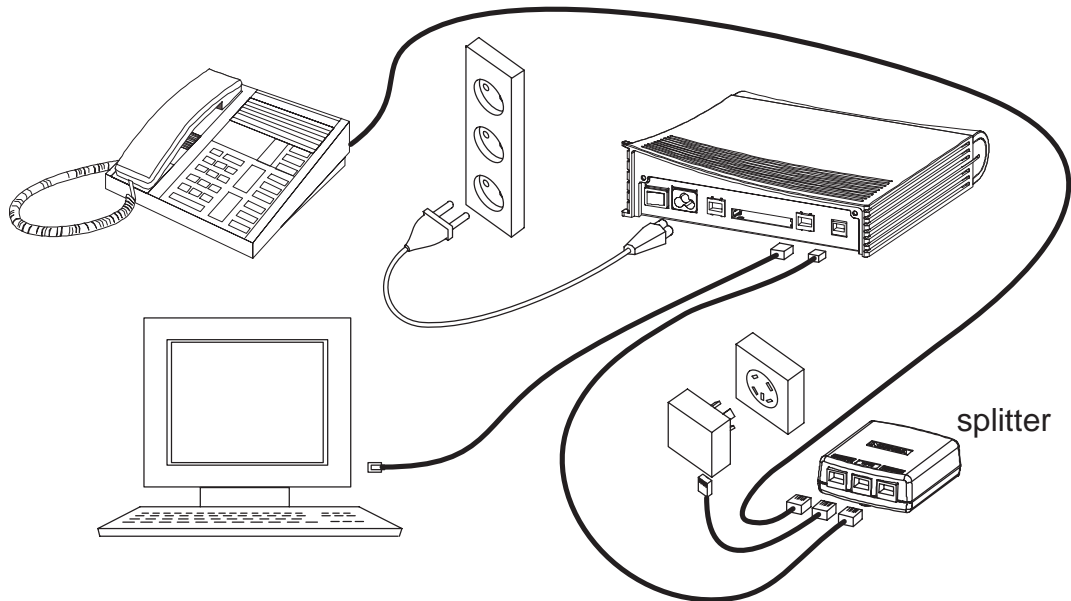
Figure 4 MW1122 and splitter connected
