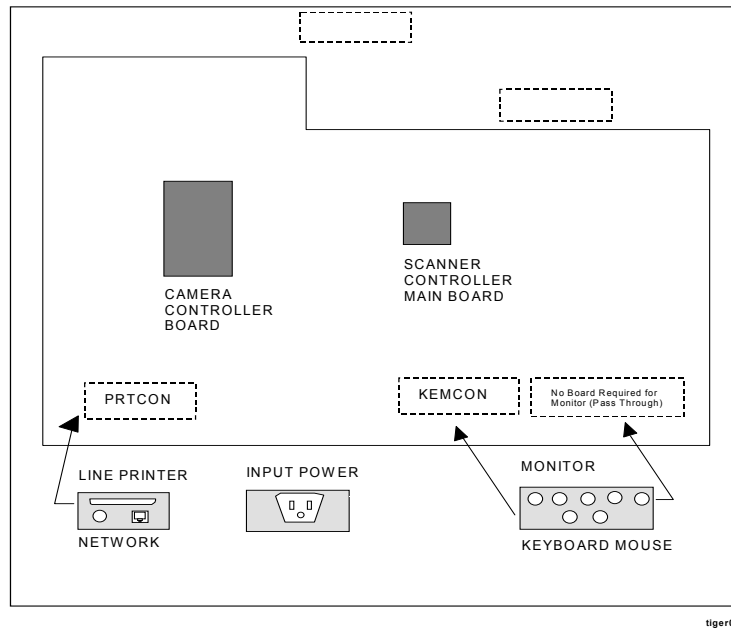
Figure 3 – 2: Standalone Board/Connector Locations
