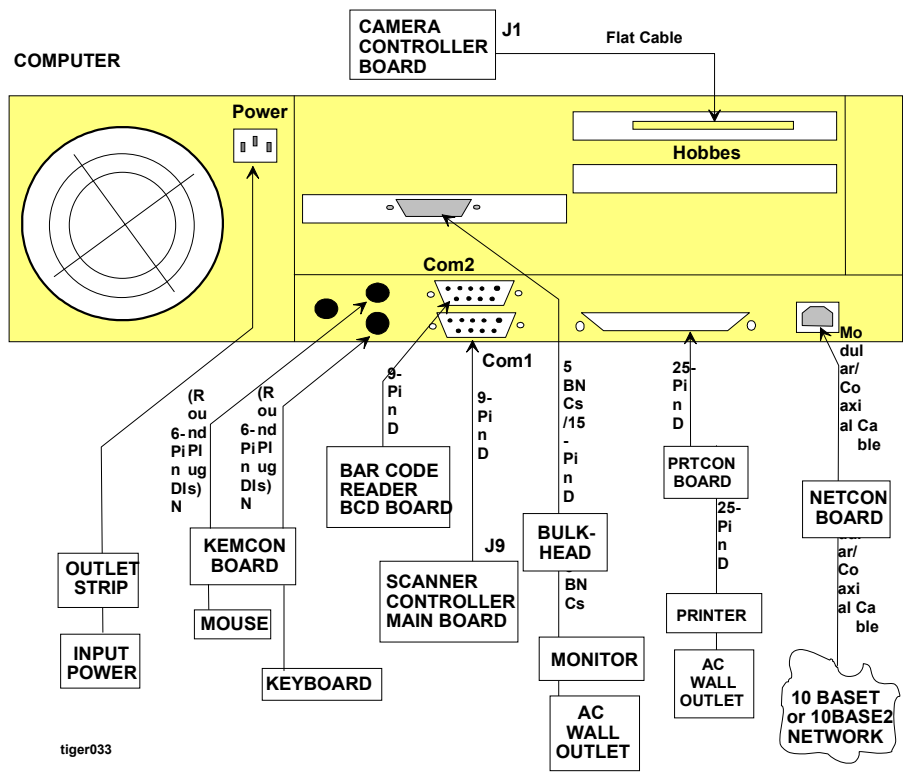
Figure 3 – 5: Computer and PC Board Connections{ XE "PC boards" }
