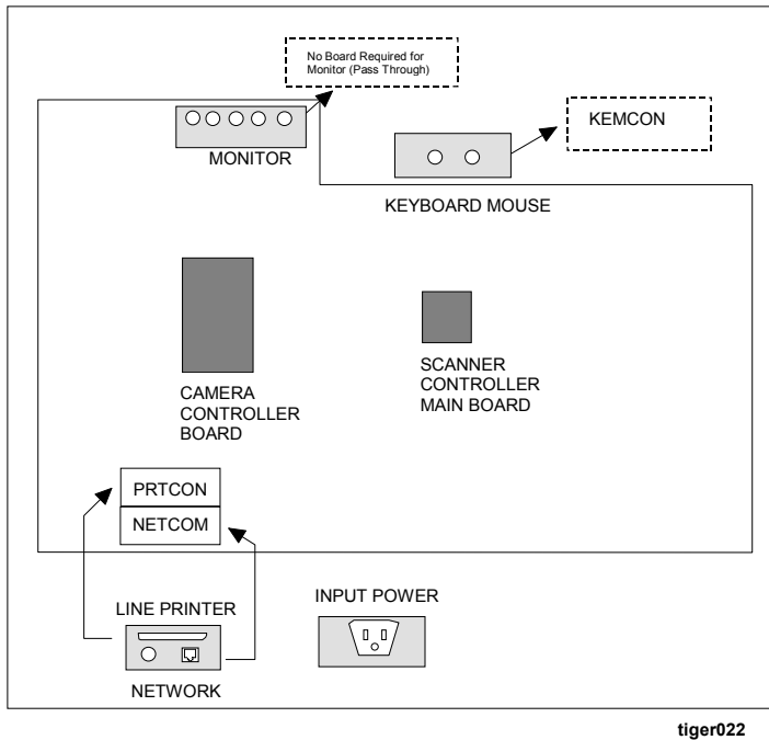
Figure 3 – 4: Network Board/Connector Locations
