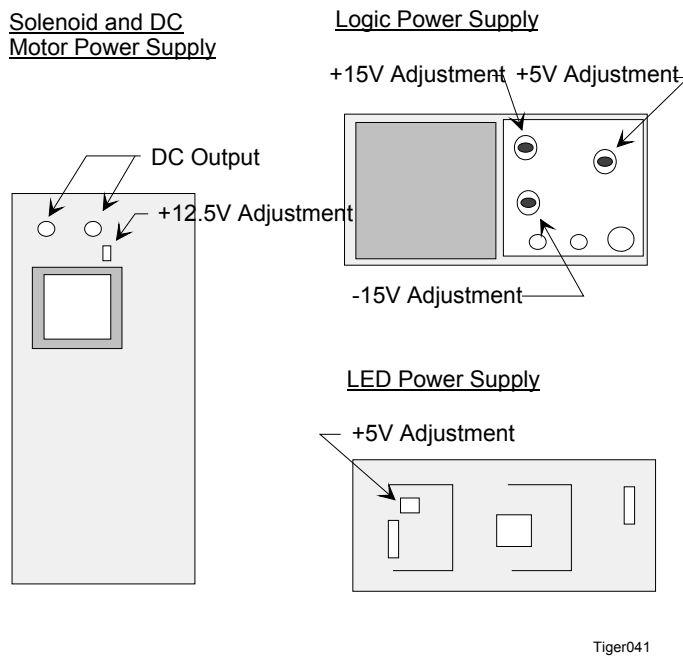
Figure 2 - 2: Adjustment Locations
