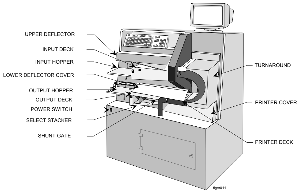
Figure 1 – 1: Scanner Parts
