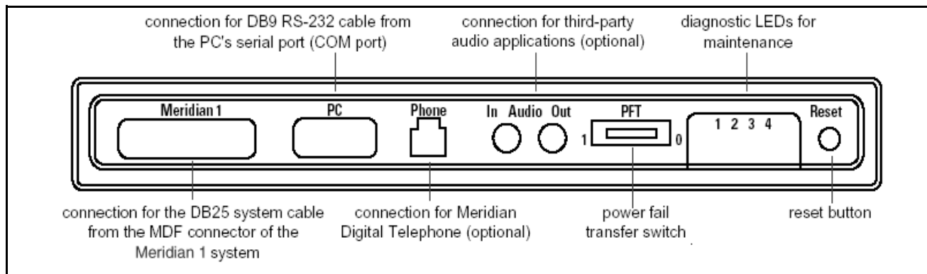
Figure 2: Back panel of the PC Console Interface Unit
