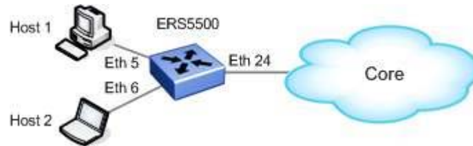
Figure 5: Traffic Meter Example
