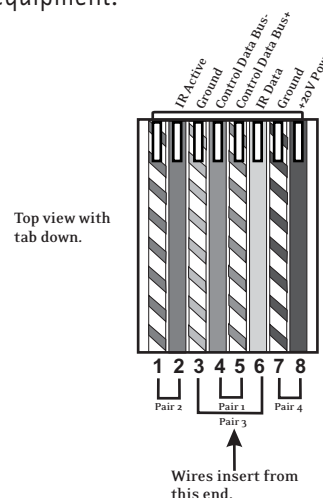
Fig. 1: EIA 568A and 568B wiring scheme for CAT5 Cable
