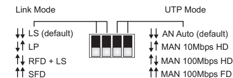
Figure 1: DIP-switch Configurations
