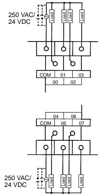
CPM1A-8ER
