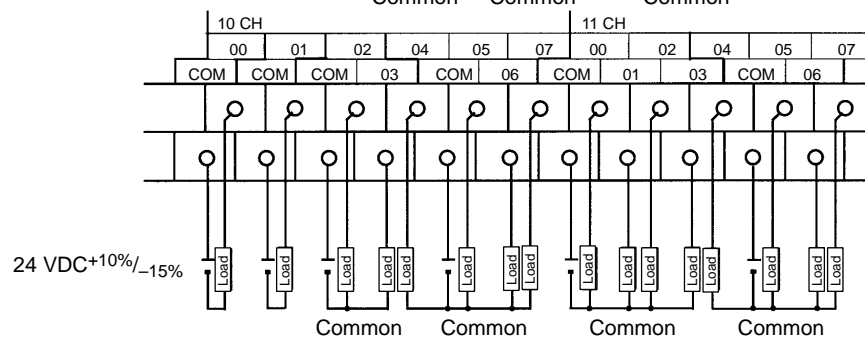
CPM1A-40CDT1-D
