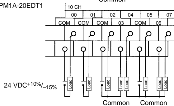
CPM1A-20CDT1-D/CPM1A-20EDT1
