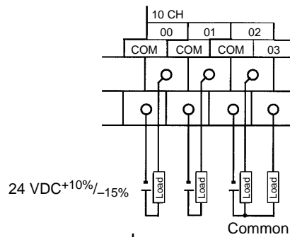
CPM1A-20CDT-D/CPM1A-20EDT
