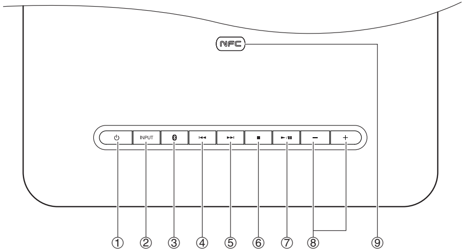
Front Panel
