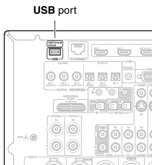
USB port
