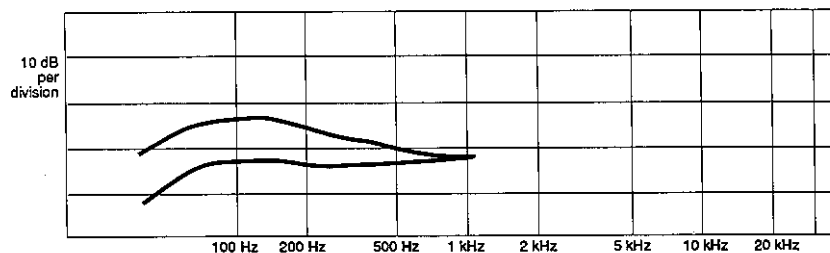
0° & 180° FREQUENCY RESPONSE
