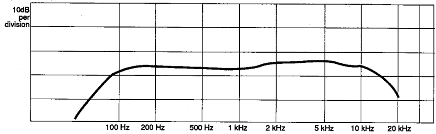
FREQUENCY RESPONSE
