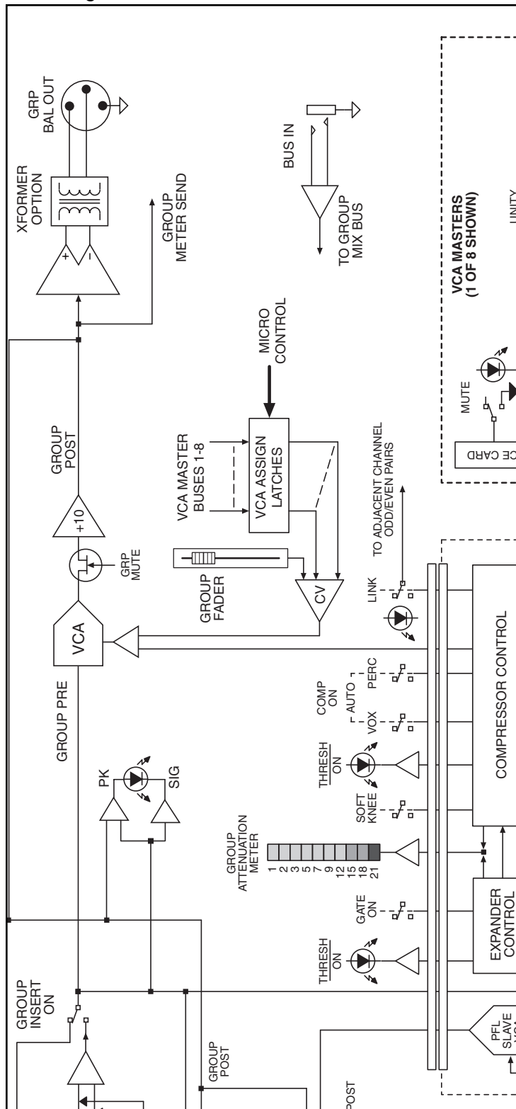
block diagram
