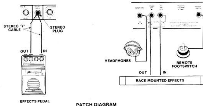
PATCH DIAGRAM
