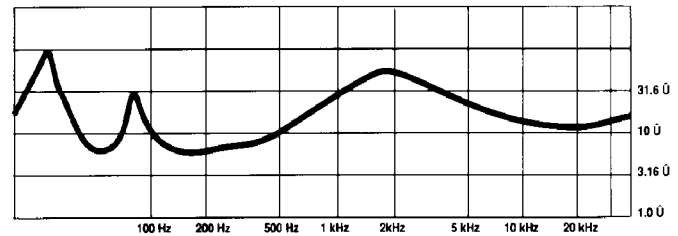
Figure 2. IMPEDANCE
