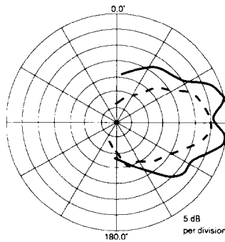
Figure 3. POLAR PATTERNS
