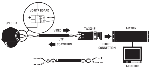
Figure 1. TW3001P Basic Applications
