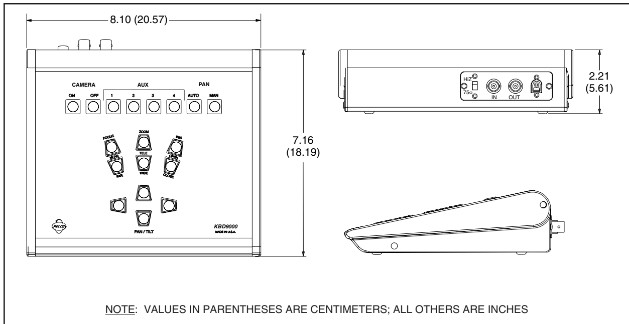
Figure 6. KBD9000 Dimension Drawing
