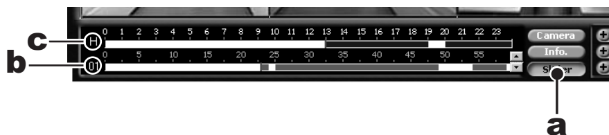
Figure 28. Slider Search
