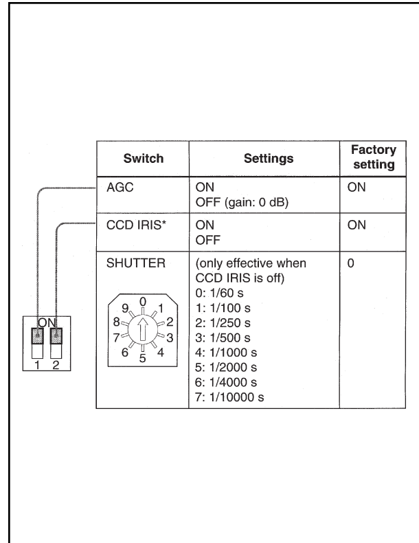
Figure 3. Internal Switch Settings
