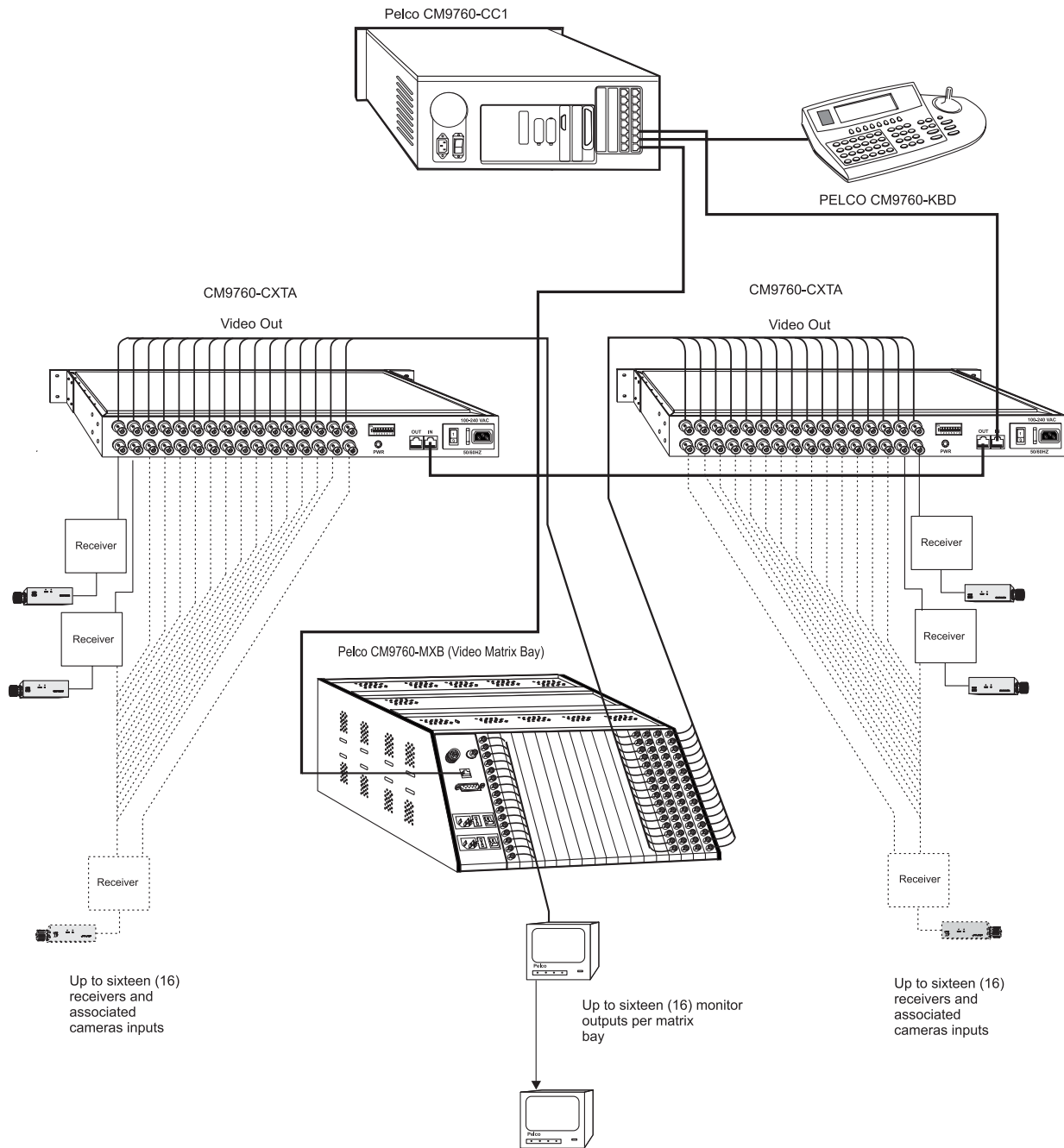
Figure 14. 9760 System Installation
