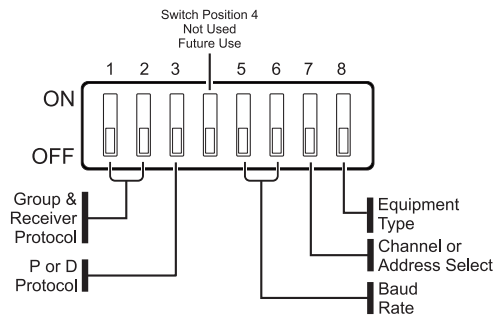
Figure 5. Configuration Switch
