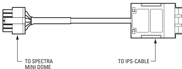
Figure 1. IPS-MINIADPT Cable
