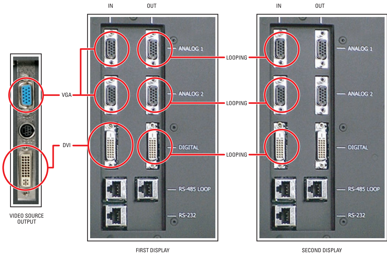
Figure 6. Video Input Connections
