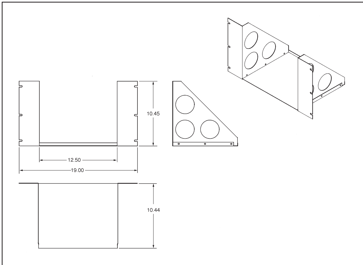
Figure 1. RMA13 Dimension Drawing
