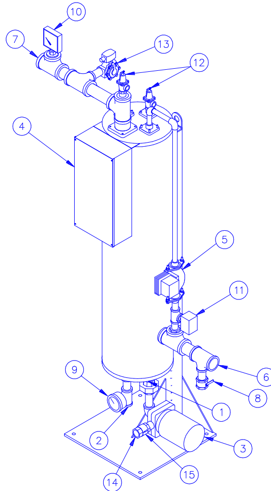
TYPICAL CONSTRUCTION FIGURE 24-1
