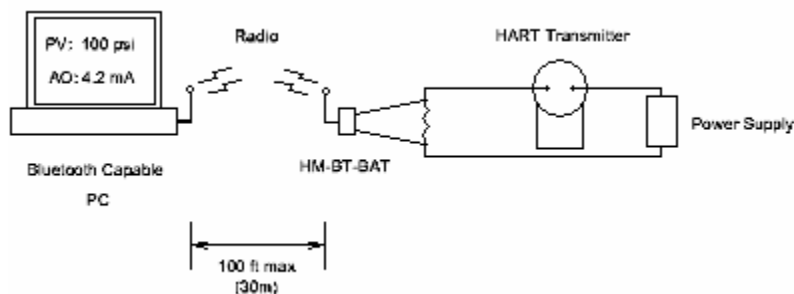
Figure 1. Bluetooth System Diagram
