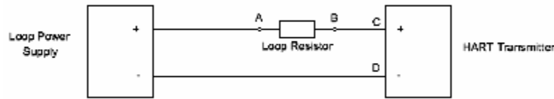
Figure 2. HART Connections
