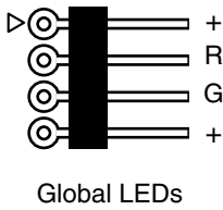
Figure 8. Global and Aggregate LED pins, EX4650A and EX8650A
