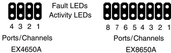
Figure 7. Global and Aggregate LED pins, EX4650 and EX8650
