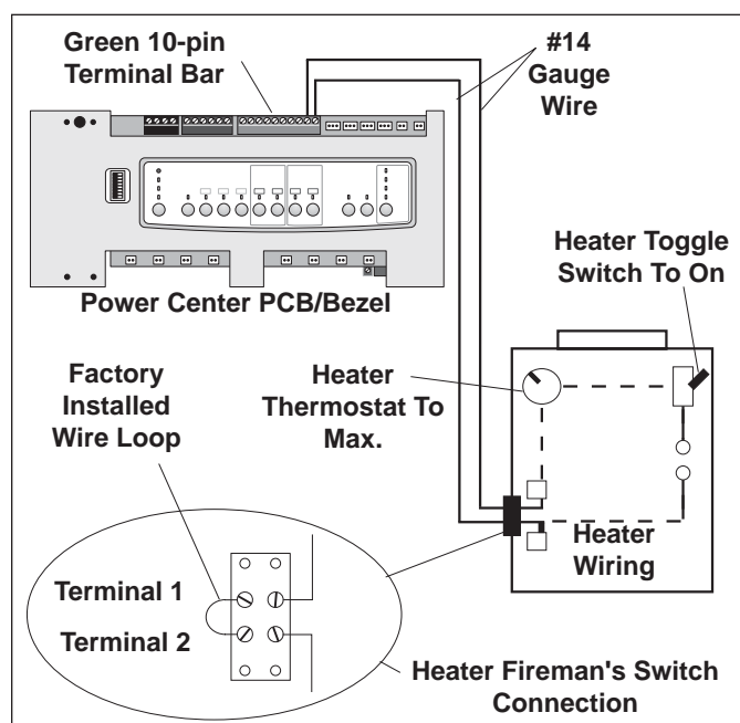
Figure 9. Lite2 Heater Connection
