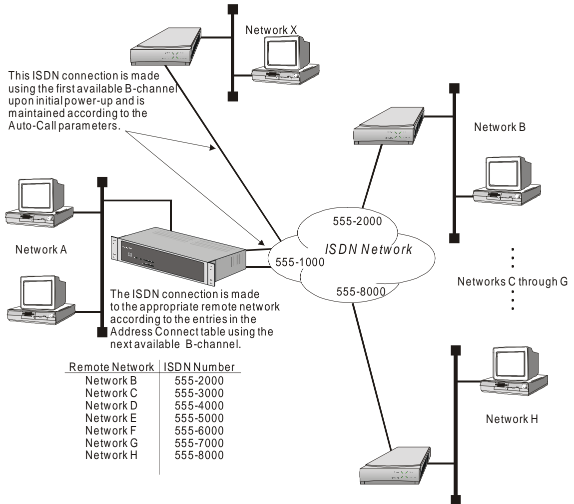
Figure 2 - 3 Auto-Call & Address Connect WAN Topology
