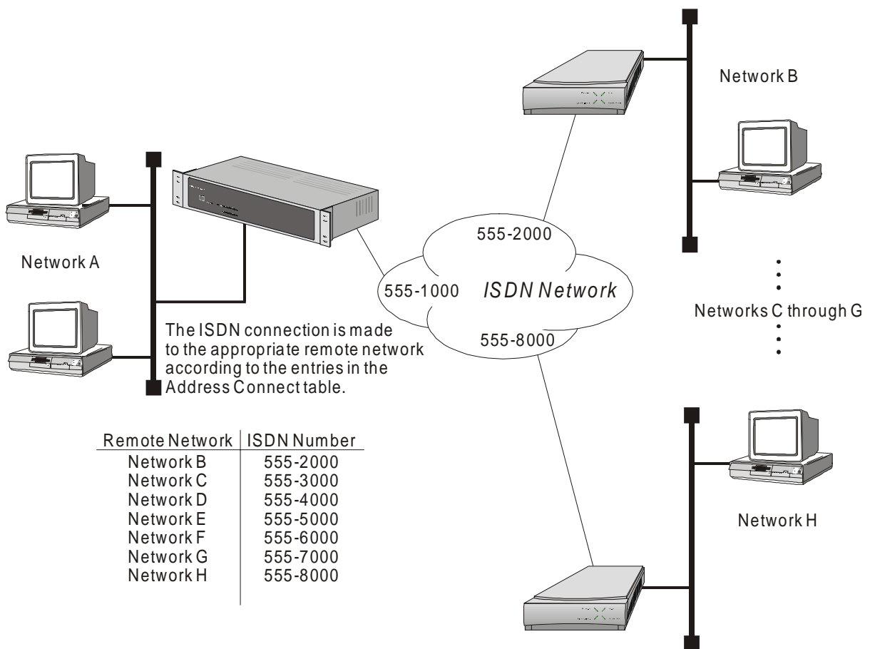
Figure 2 - 2 Address Connect WAN Topology
