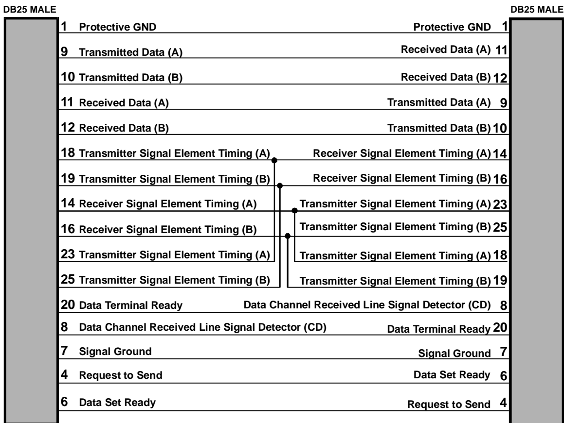
Figure 3 – 11 V.35 Null-Modem Cable
