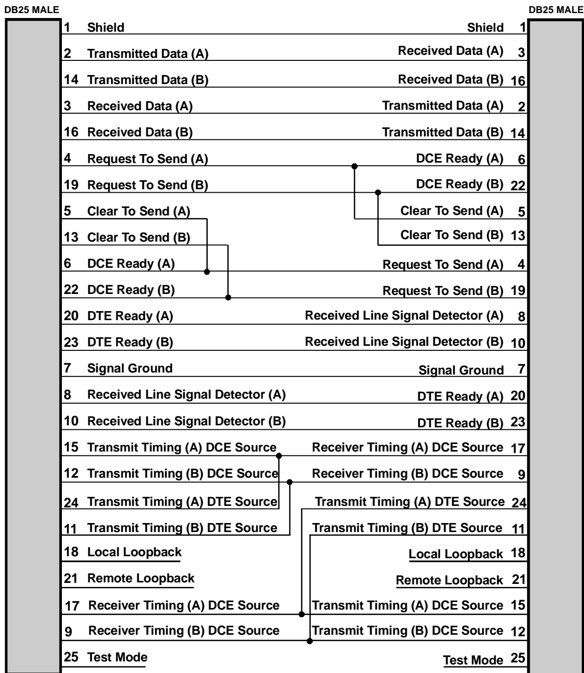
Figure 3 – 12 RS530 Null-Modem Cable
