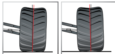
Positive Camber Negative Camber
