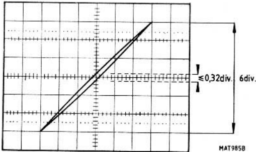
Figure 4.2 Phase shift
