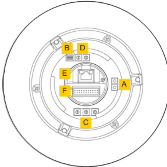
Outdoor Dome
