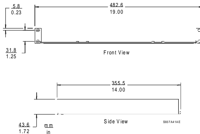
Rack Kit
