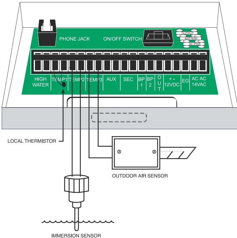
Fig. 2.4 Connecting Temperature Sensors
