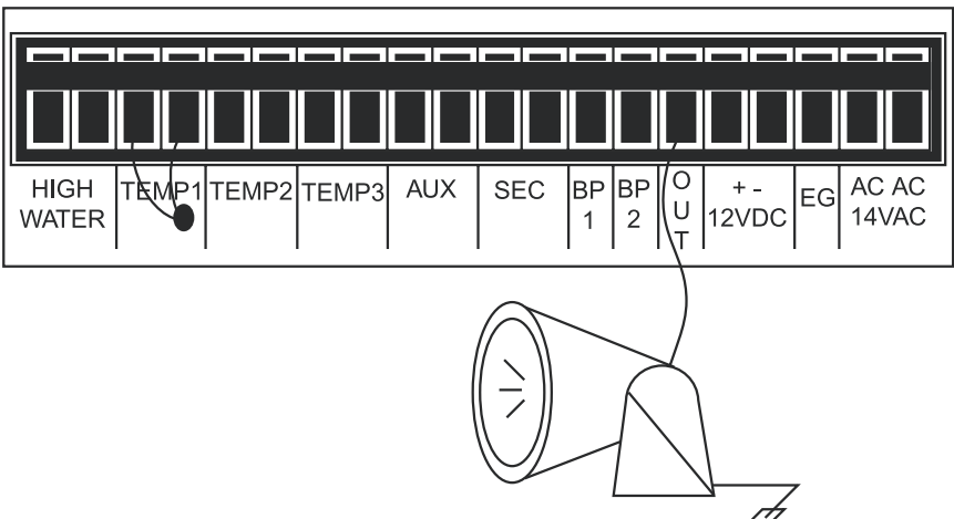
Fig. 2.8 Connecting a Strobe Light to the Output
