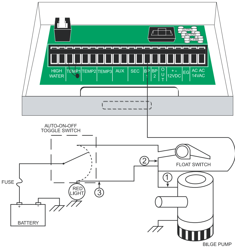
Fig. 2.5 Connecting the Bilge Pump
