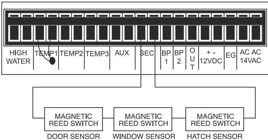
Fig. 2.6 Connecting Accessories to the Security Input
