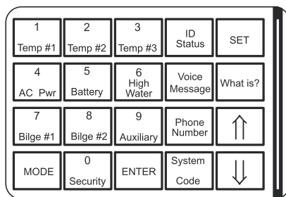
Fig. 3.1 The Keypad
