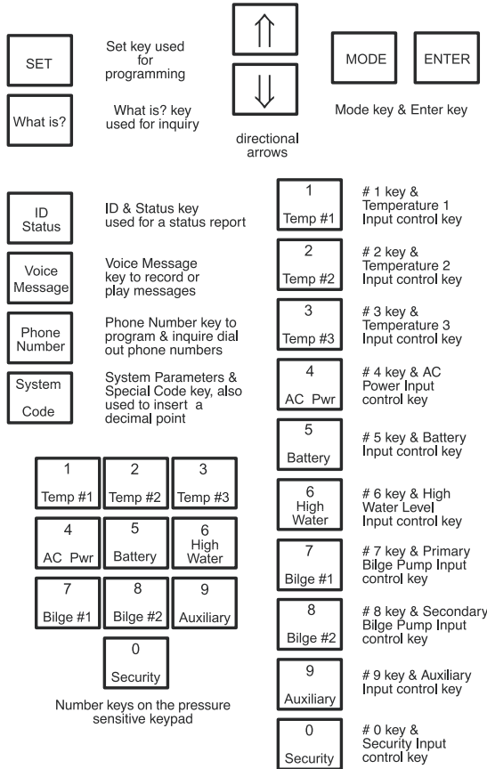
Fig. 3.2 The Keypad Keys and Their Functions
