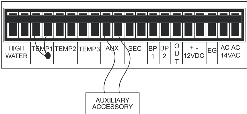
Fig. 2.7 Connection to the Auxiliary Input
