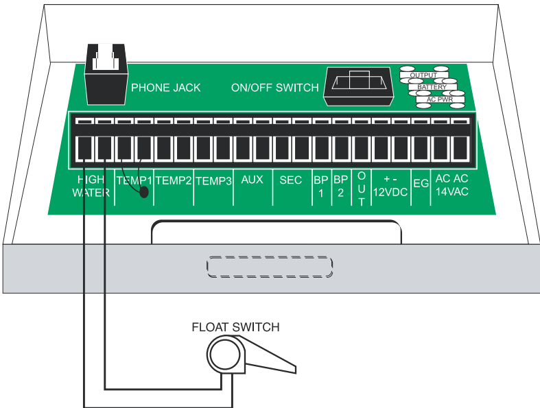
Fig. 2.3 Connecting the High Water Float Switch
