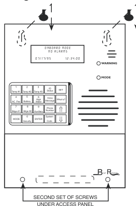
Fig. 2.1 Mounting the Boat Remote
