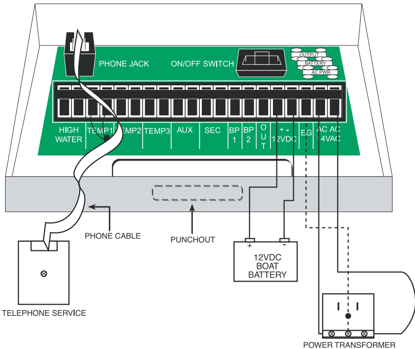
Fig. 2.2 Connecting Power and Telephone Service
