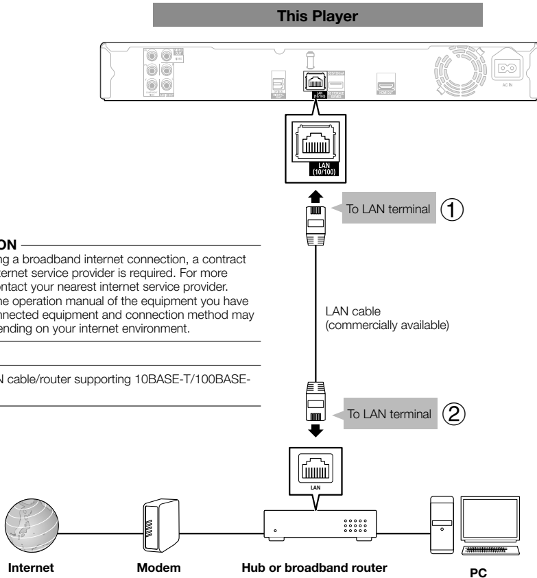
Example of a Broadband Internet Connection
