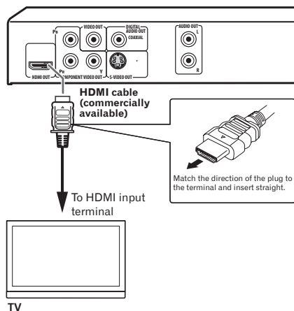
Player's rear panel
