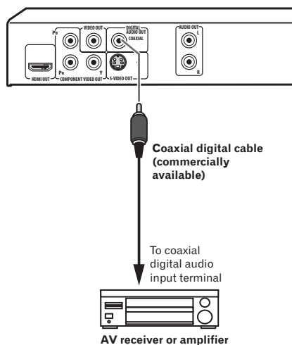
Player's rear panel
