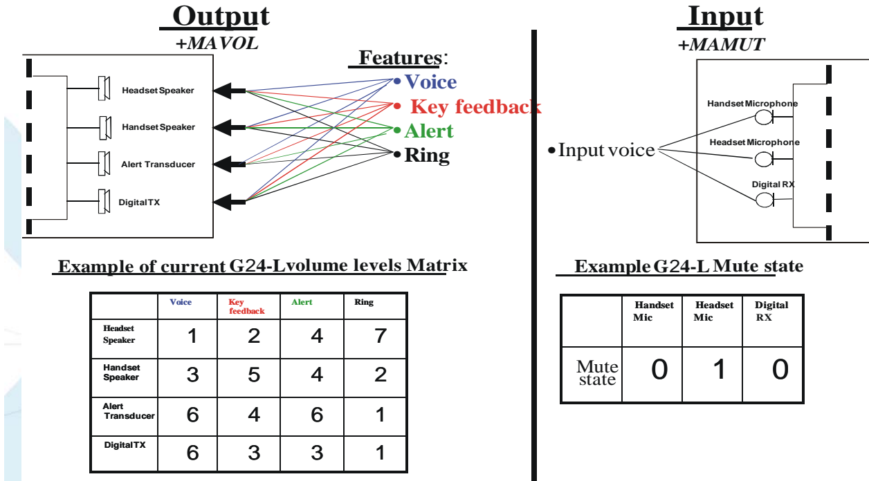
Figure 3-7: G24-L Audio Gain
