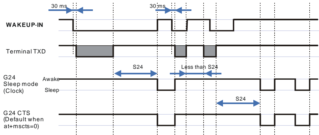
Figure 3-11: Sleep Mode when S24 > 0
