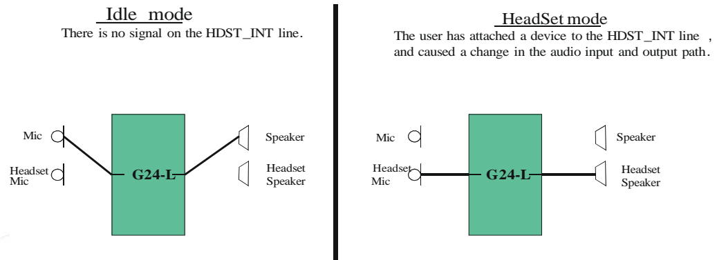
Figure 3-3: Basic Audio Setup
