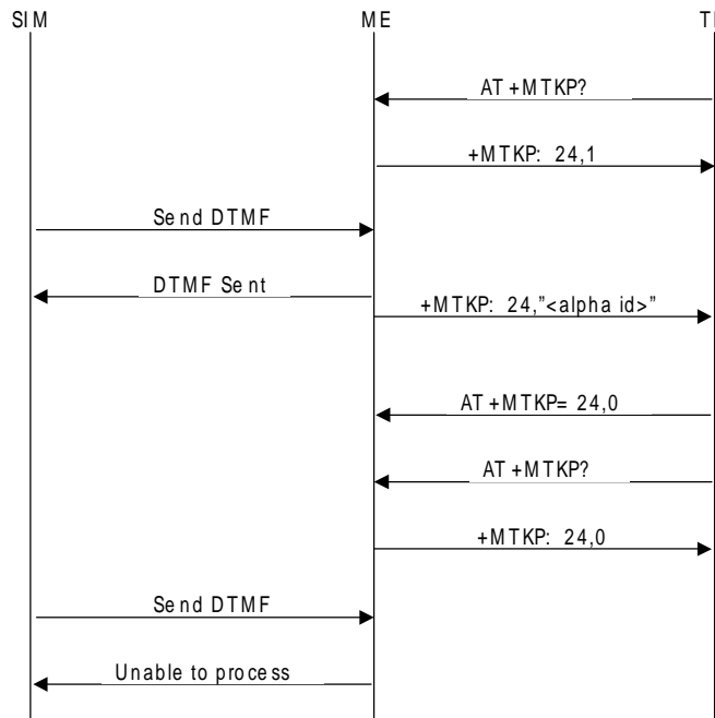
Figure 3-14: Communication During DTMF Command
