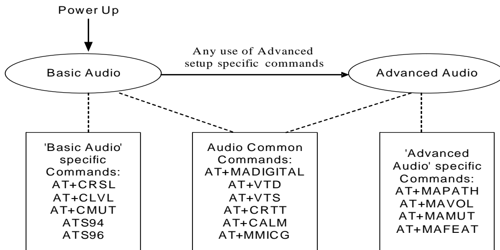
Figure 3-2: Audio Modes
