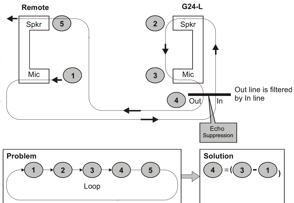
Figure 1-3: Echo Suppression
