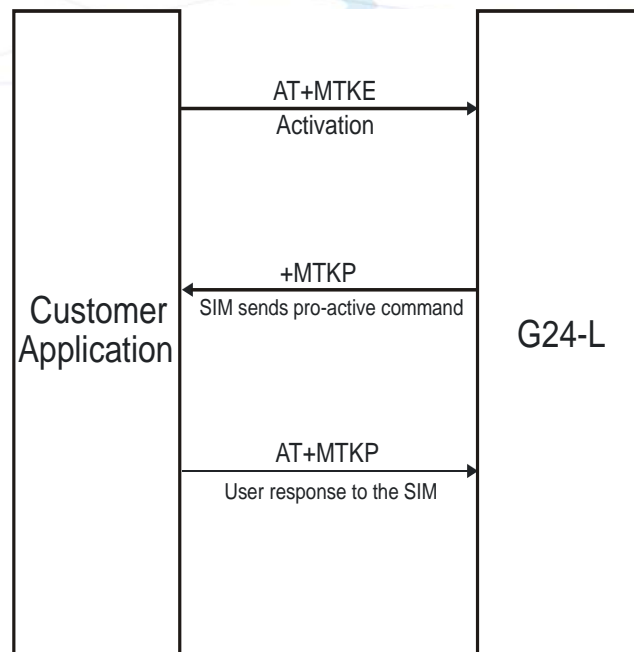
Figure 3-13: SIM Toolkit
