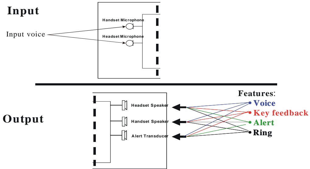
Figure 3-6: Audio Paths
