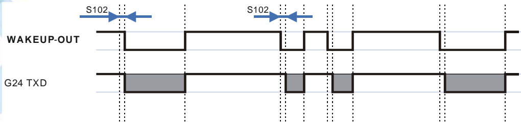
Figure 3-12: G24-L Lines when S24 > 0
