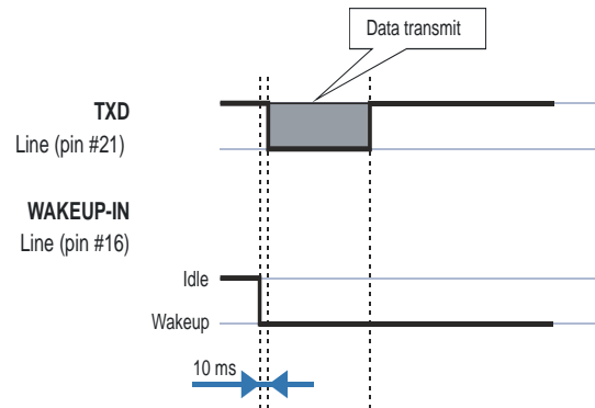
Figure 3-9: Wakeup-In Line
