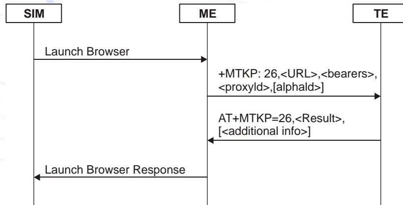
Figure 3-15: Communication During Launch Browser Command
