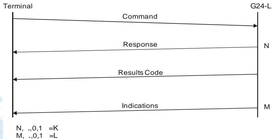
Figure 2-1: AT Commands Protocol
