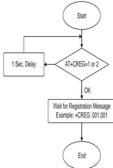
Figure 4-8: G24-L Network Connection
