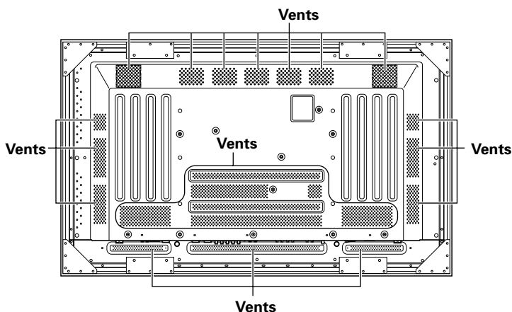
Illustration depicts PRO-100HDI model.
