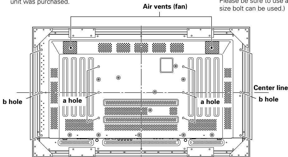
Rear view diagram (PRO-1000HDI)
