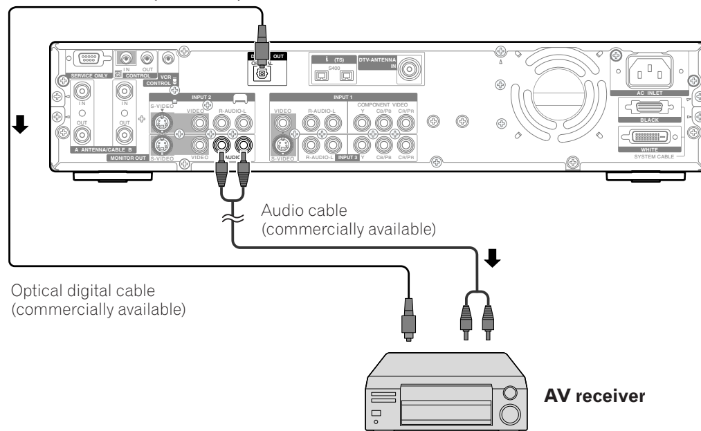
Media Receiver (rear view)
