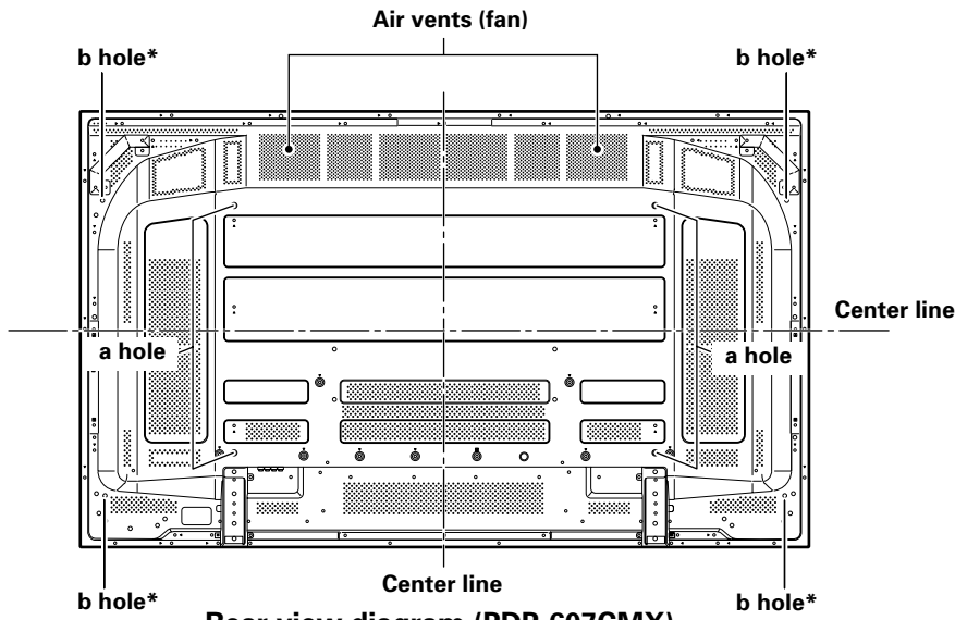
Rear view diagram (PDP-607CMX)
