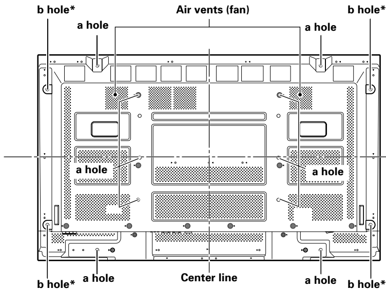
Rear view diagram (PDP-507CMX)
