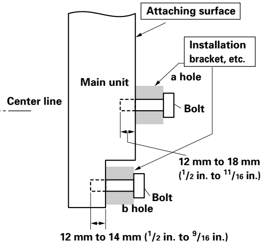
Side view diagram
