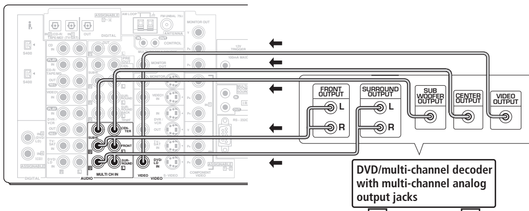
Note that the illustration above shows the VSX-2014i however, connection for the VSX-1014 is the same.
