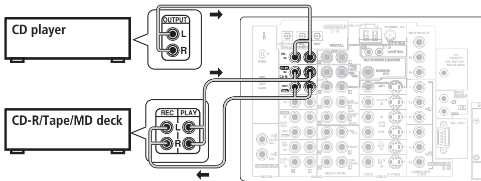
Note that the illustration above shows the VSX-2014i however, connection for the VSX-1014 is the same.
