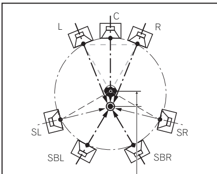
The central axes converge 30 cm (12 inches) to 80 cm (31 inches) behind the listening position.
