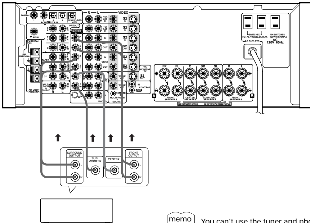
Components equipped with 5.1 channel analog output jacks
