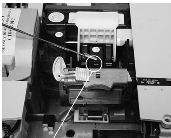
Printhead stand-off
