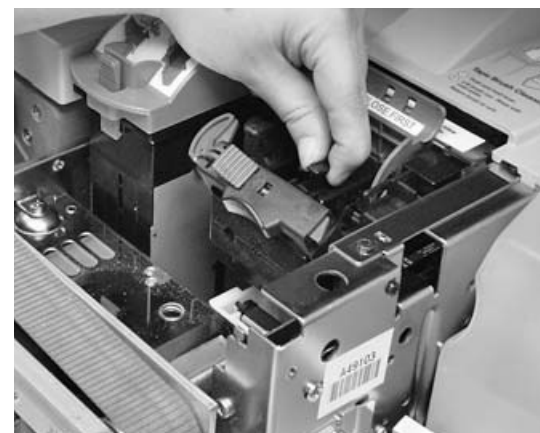
Printhead Standoff
