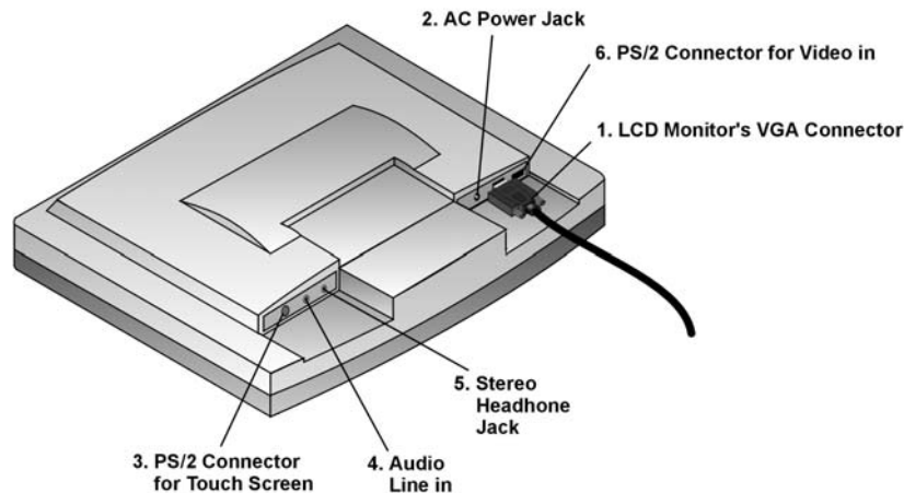
Figure 1-2: LCD Monitor's Rear Ports
