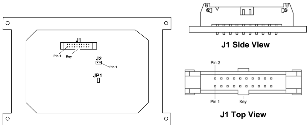
Figure 2. AM8 Data/Power Connector
