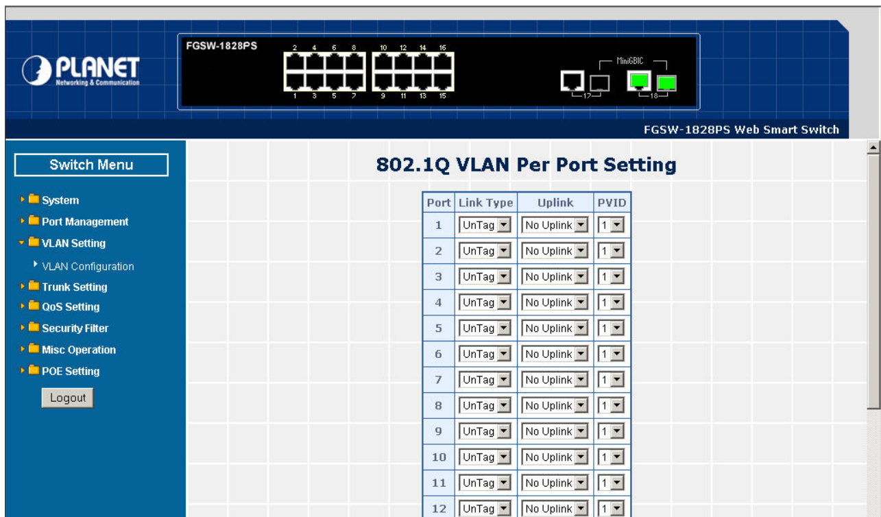
Figure 4-29 802.1Q VLAN per Port Setting Web Page Screen
