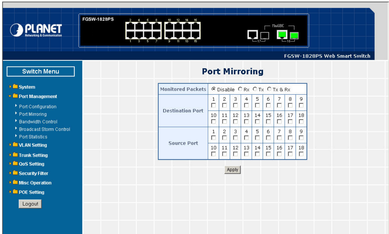
Figure 4-22 Port Mirroring Web Page Screen
