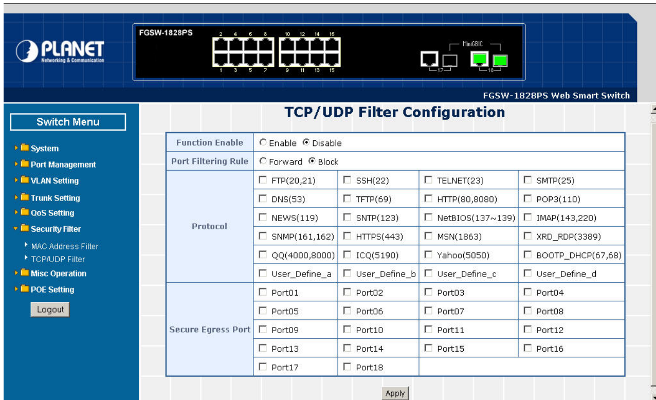
Figure 4-50 TCP / UDP Filter Web Page Screen
