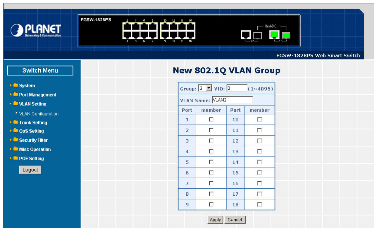
Figure 4-31 Add new VLAN Group Screen
