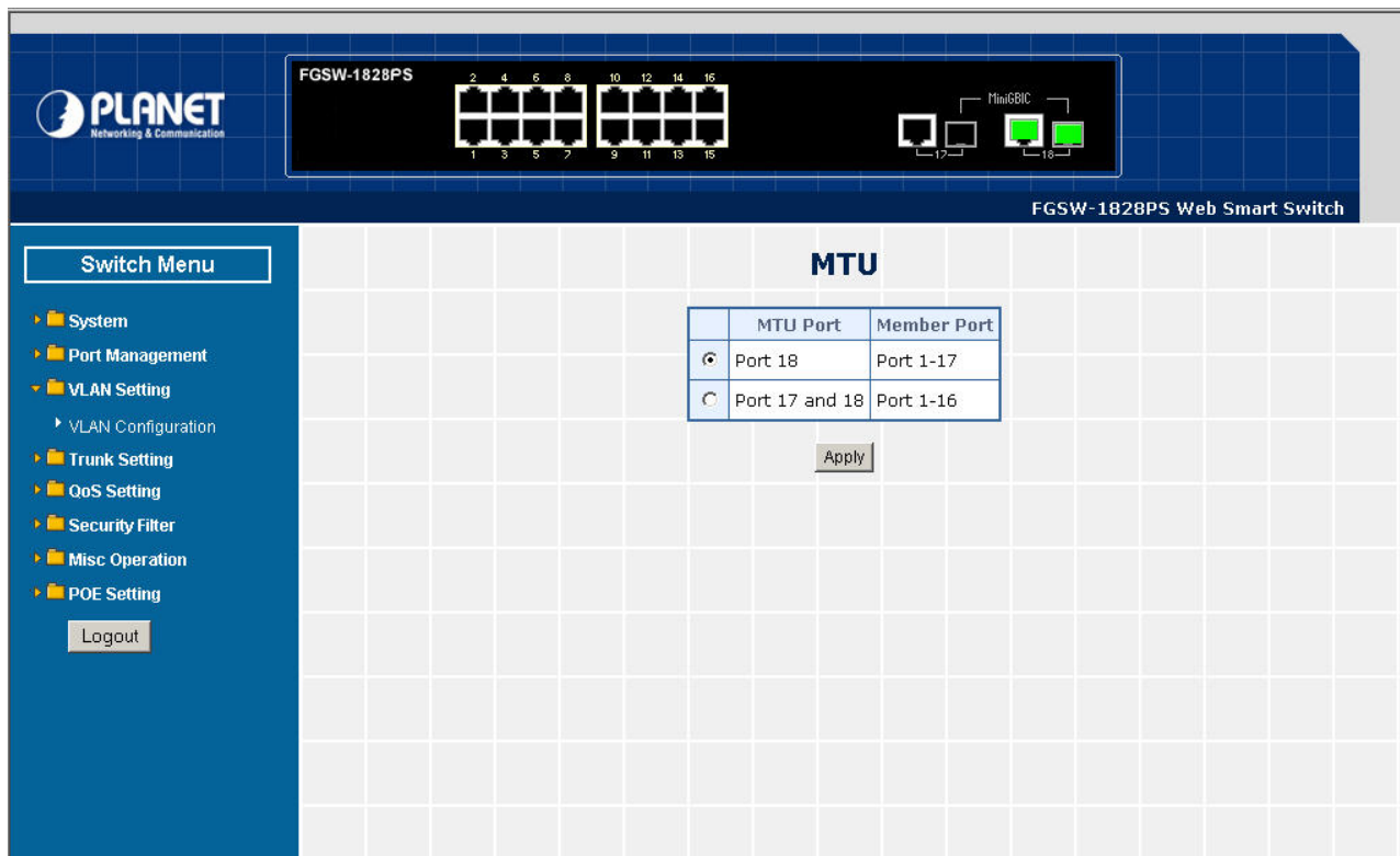
Figure 4-41 MTU VLAN Configuration Web Page Screen
