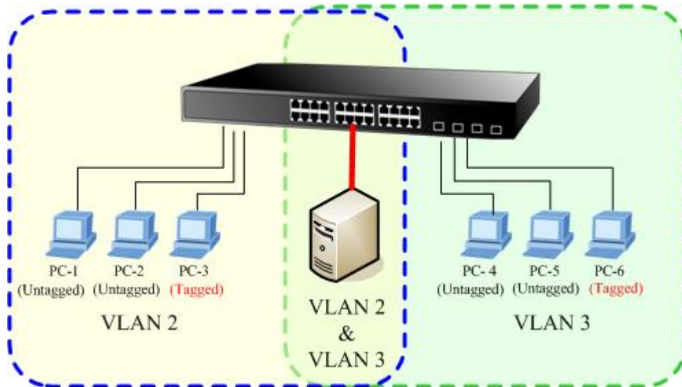
Figure 4-35 A Server connect to the VLAN overlapping area
