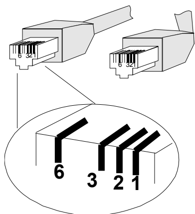
The standard RJ-45 receptacle/connector
