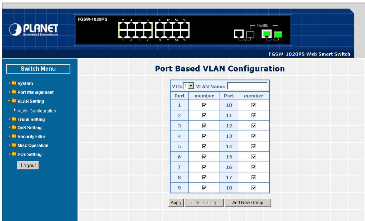
Figure 4-40 Port Based VLAN Configuration Web Page Screen
