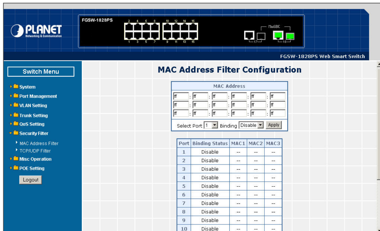
Figure 4-48 Security Filter Web Page Screen
