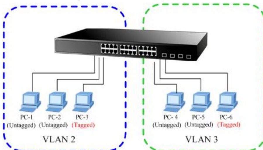
Figure 4-30 two separate 802.1Q VLAN diagram
