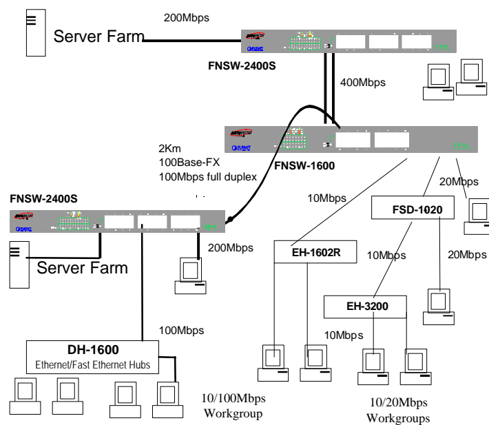
Figure 3: Sample Application for the Switch with Trunk
