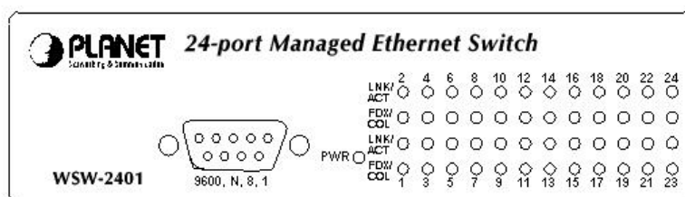
Figure 2-2 LED Indicators
