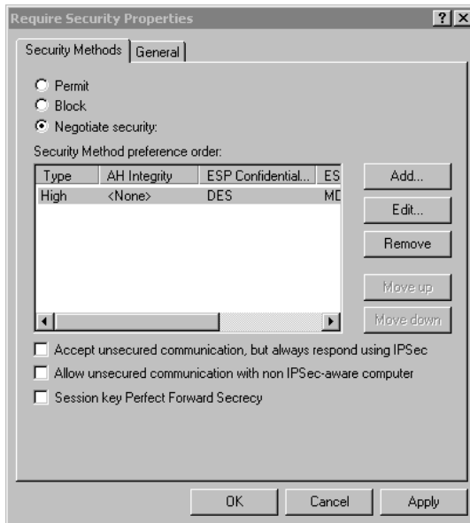
Figure76: Security Methods
