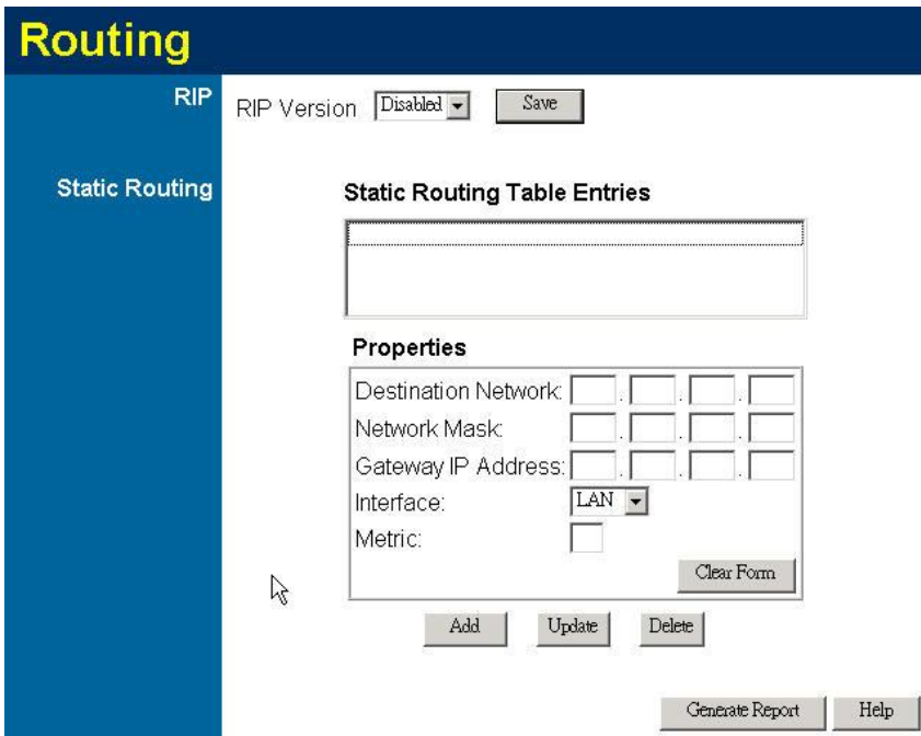
Figure119: Routing Screen
