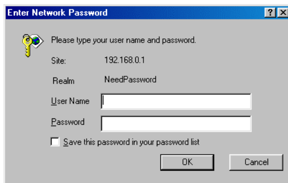
Figure 7: Password Dialog
