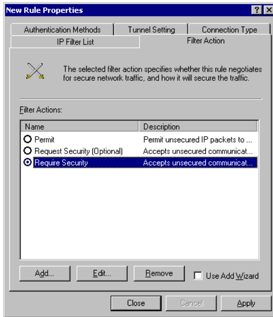
Figure75: Filter Action
