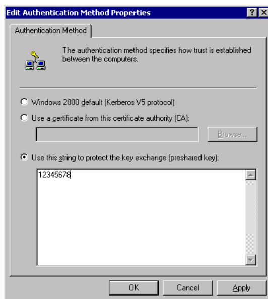
Figure70: Authentication Method
