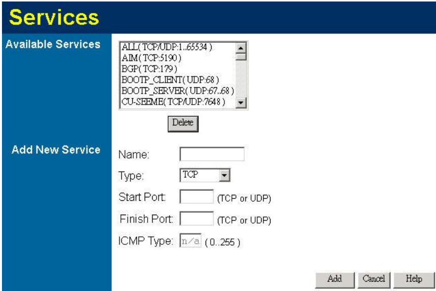
Figure46: Services Screen
